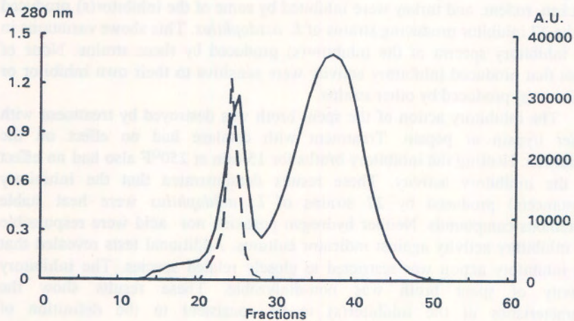
Figure 1. Elution profile of ammonium sulfate precipitate of inhibitory activity produced by L. acidophilus GP4A on Sephadex G-200. Each 5 ml fraction was monitored at 280 nm ( — ) and was assayed for inhibitory activity ( - - - ).
