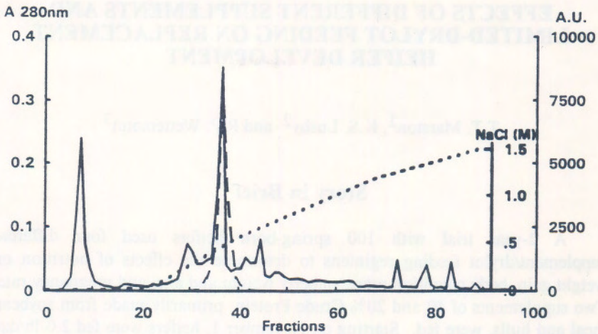
Figure 2. Chromatography of inhibitory activity obtained from Sephadex G-200 produced by L. acidophilus GP4A on DE 52 anion exchange. The activity was eluted with 0 to 1.5 M NaCl (.....). Each 4 ml fraction was monitored at 280 nm (—) and was assayed for inhibitory activity (---).
